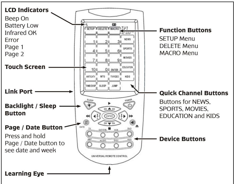
Figure 2 - 5030URC overview
