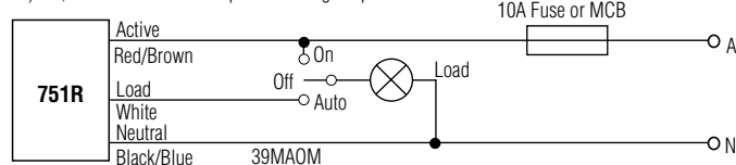
2c) ON, OFF or AUTOMATIC Operation using a 3 position switch
