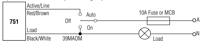
1c) ON, OFF or AUTOMATIC Operation using a 3 position switch
