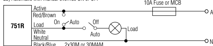
2b) Automatic with manual override ON or OFF
